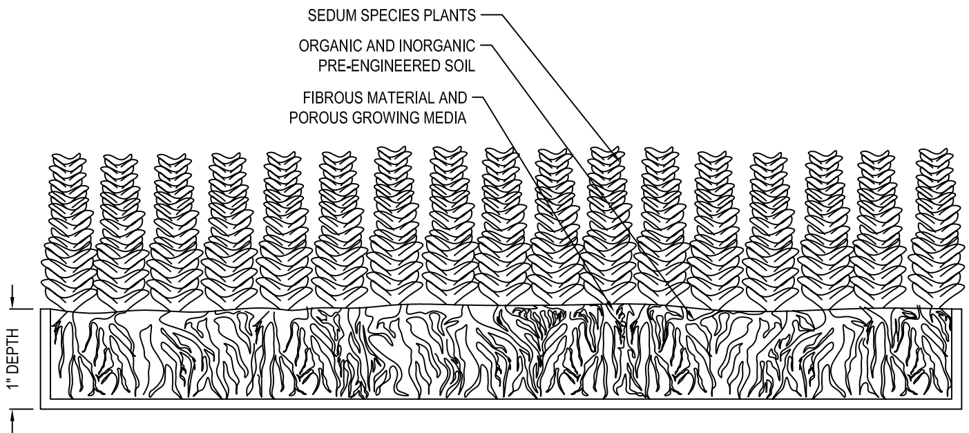
SECTION OF STANDARD SEDUM TILE
